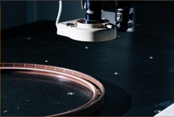
3D Vision Microscope
